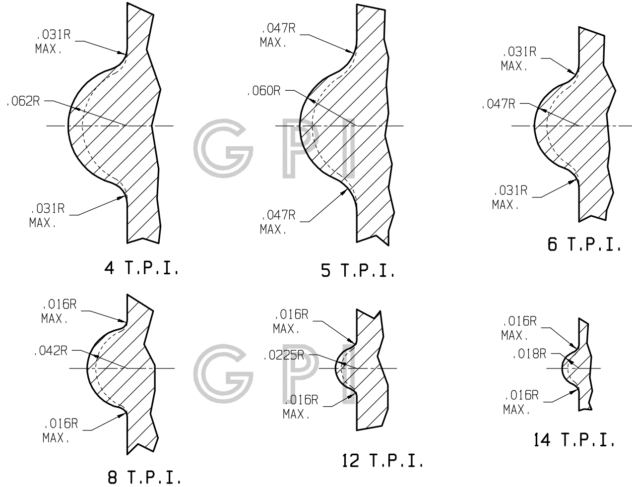
TYPICAL SAMPLES OF THREAD PROFILES
